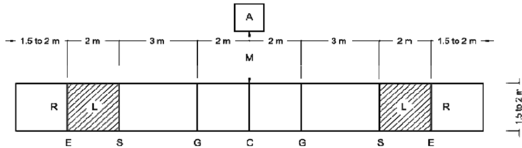
Figure 2 Standard piste for all three weapons
